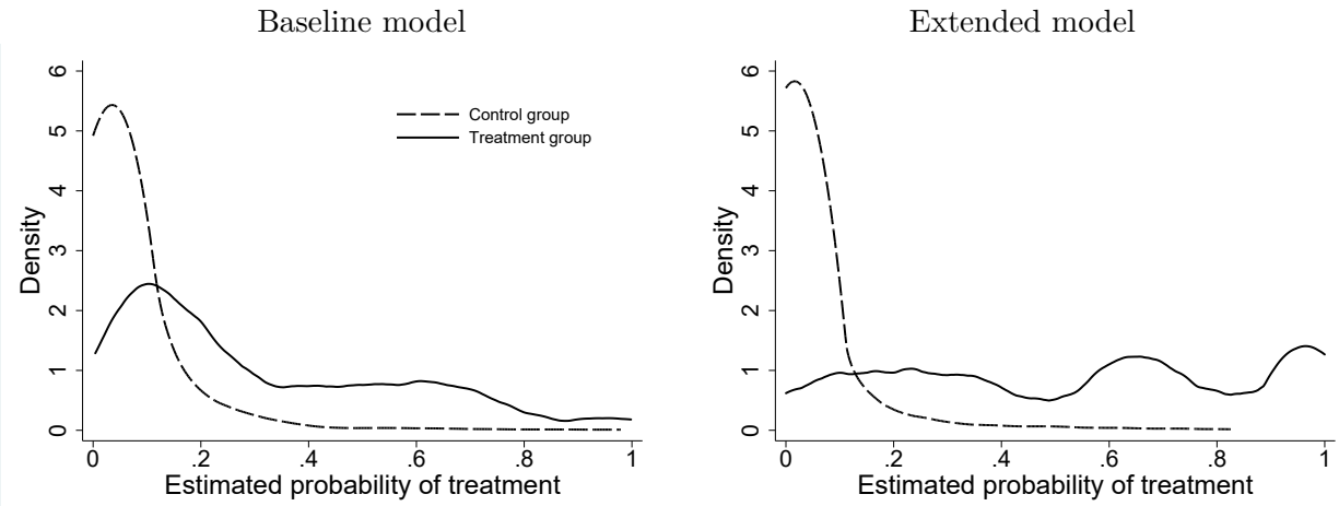
Figure A.6: Distribution of propensity score for the baseline model (left panel) and the extended model (right panel): Kernel density estimate of the predicted probabilities for treatment (solid line) and control group (dashed line) based on an Epanechnikov kernel with bandwidth 0.025.
