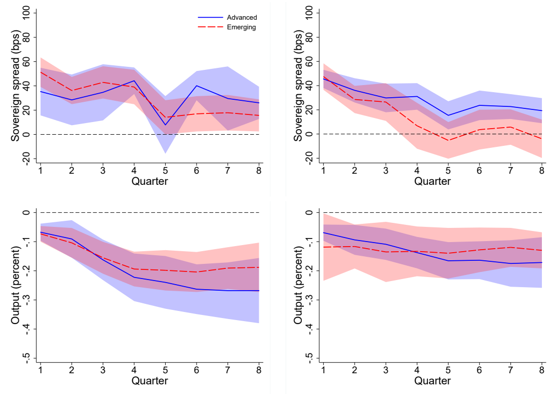
Figure A.11: Impulse responses to a h = 0 sovereign spread shock based on the ATE estimator in equation (5) together with the treatment definition in (1) when excluding Germany and the United States. For details, see Figure 9.
