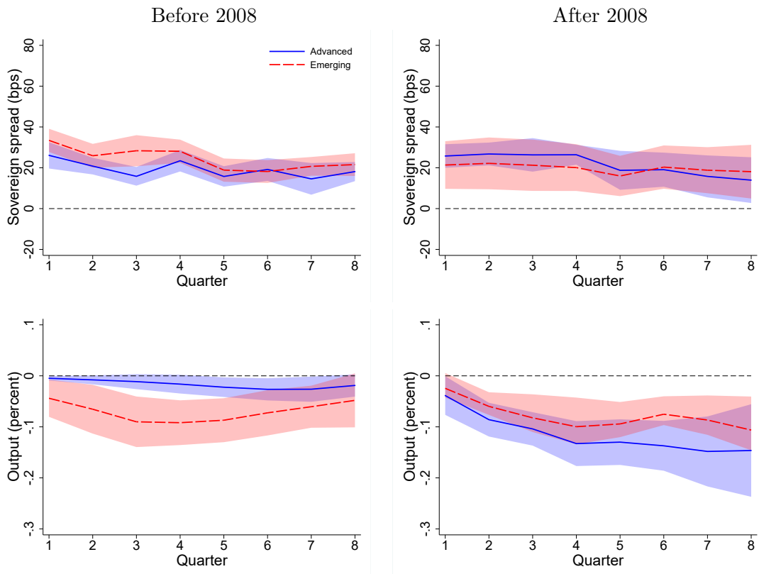
Figure A.12: Impulse responses to a country-specific sovereign spread shock based on the local projection approach with time-fixed effect added to both estimation stages. See Figure 12 for details.
